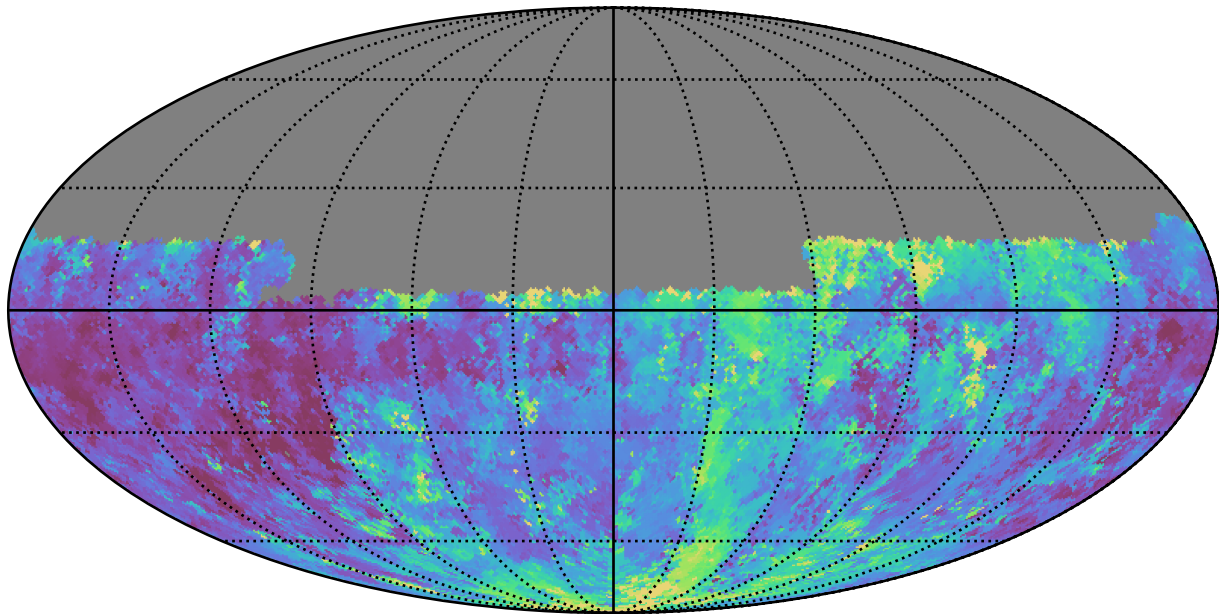
baseline_v3.5_10yrs Yr 1 u band: Median seeingEff
