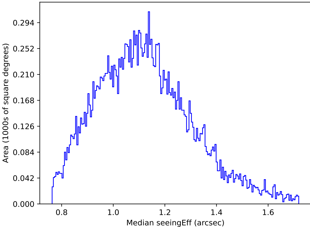
baseline_v3.5_10yrs Yr 1 u band: Median seeingEff
