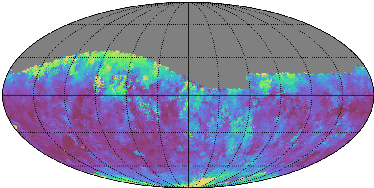
baseline_v3.5_10yrs Yr 1 r band: Median seeingEff
