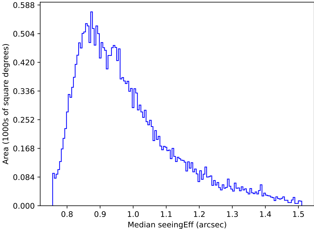
baseline_v3.5_10yrs Yr 1 r band: Median seeingEff
