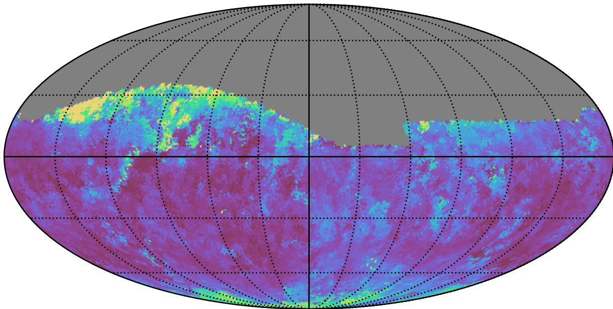
baseline_v3.5_10yrs Yr 1 i band: Median seeingEff
