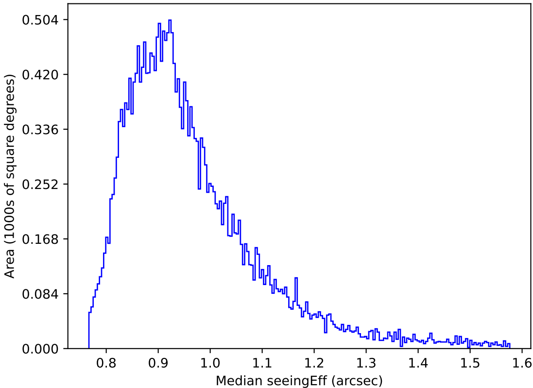
baseline_v3.5_10yrs Yr 1 i band: Median seeingEff
