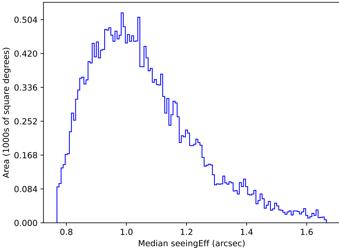
baseline_v3.5_10yrs Yr 1 g band: Median seeingEff
