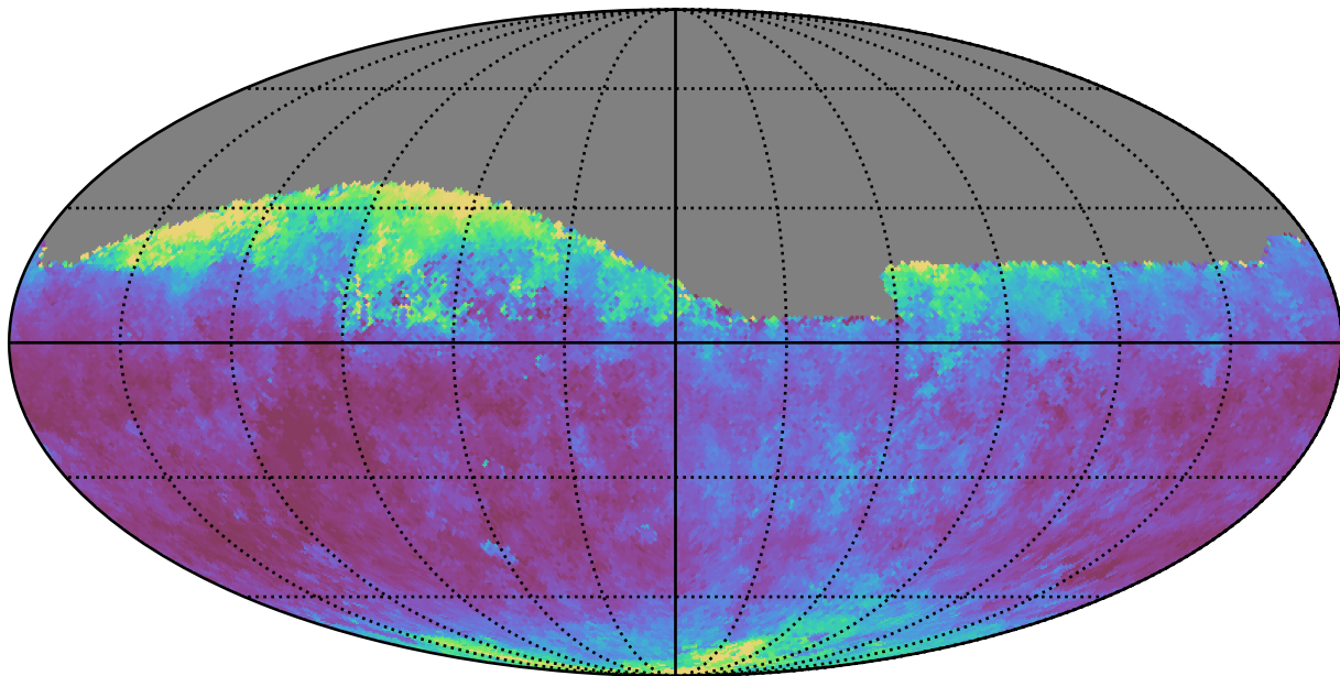
baseline_v3.5_10yrs Yr 1 all bands: Median seeingEff
