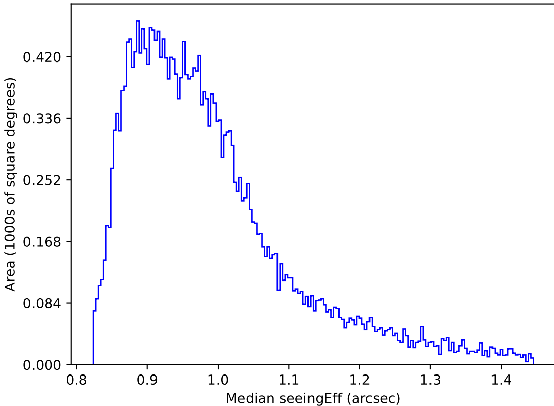
baseline_v3.5_10yrs Yr 1 all bands: Median seeingEff
