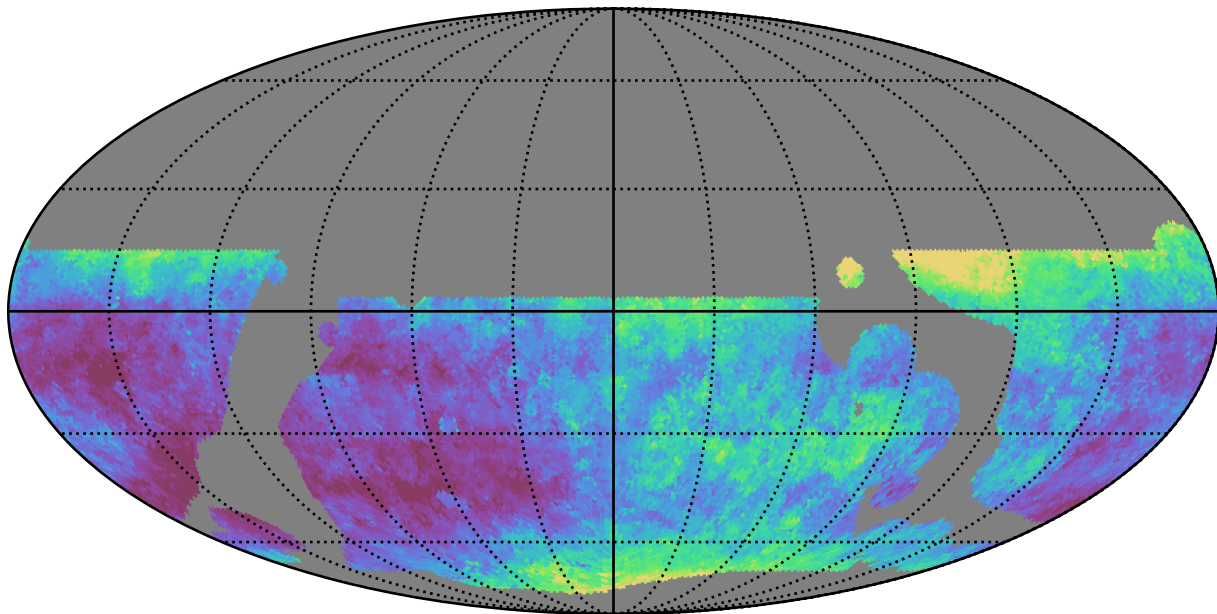
baseline_v3.5_10yrs WFD z band: Median seeingEff
