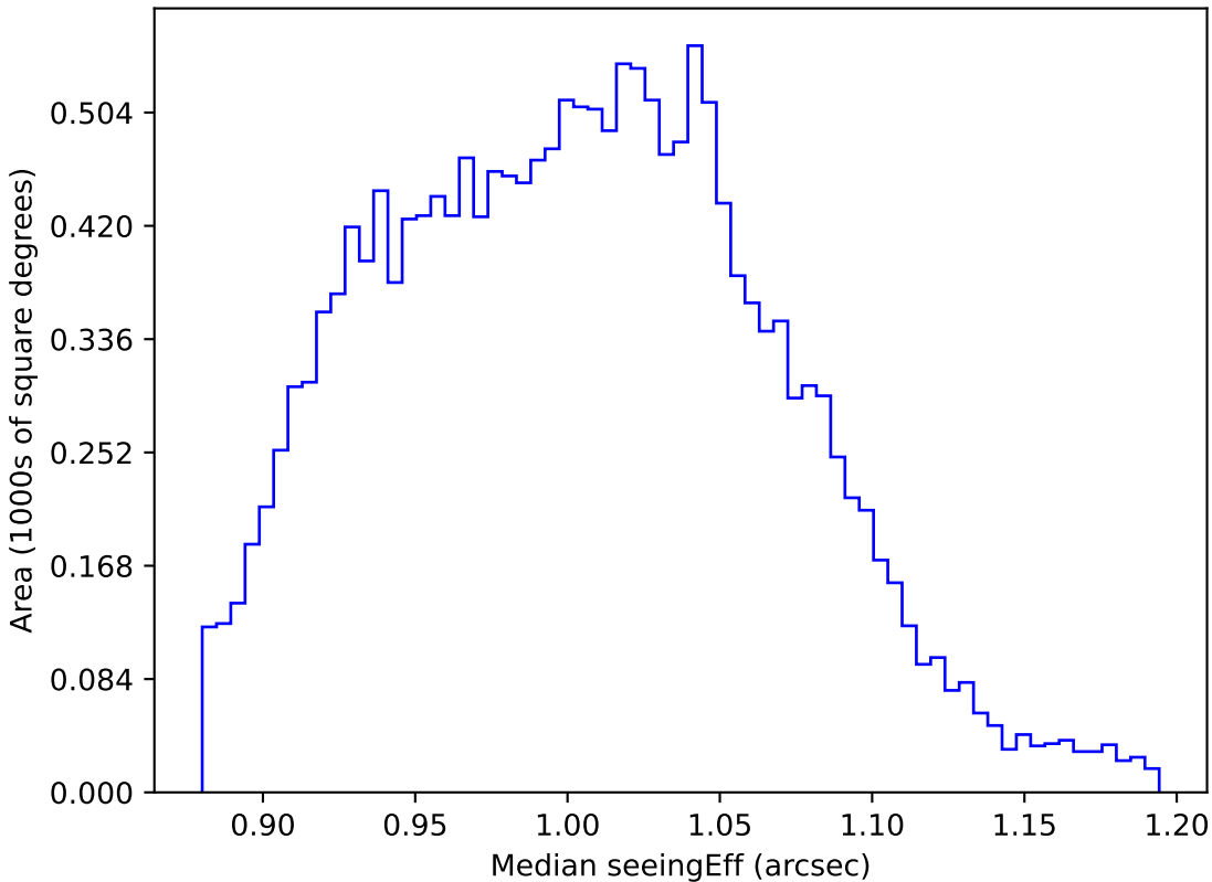
baseline_v3.5_10yrs WFD z band: Median seeingEff
