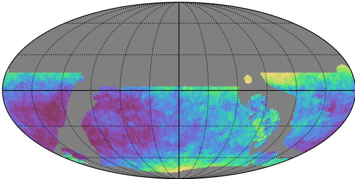
baseline_v3.5_10yrs WFD y band: Median seeingEff
