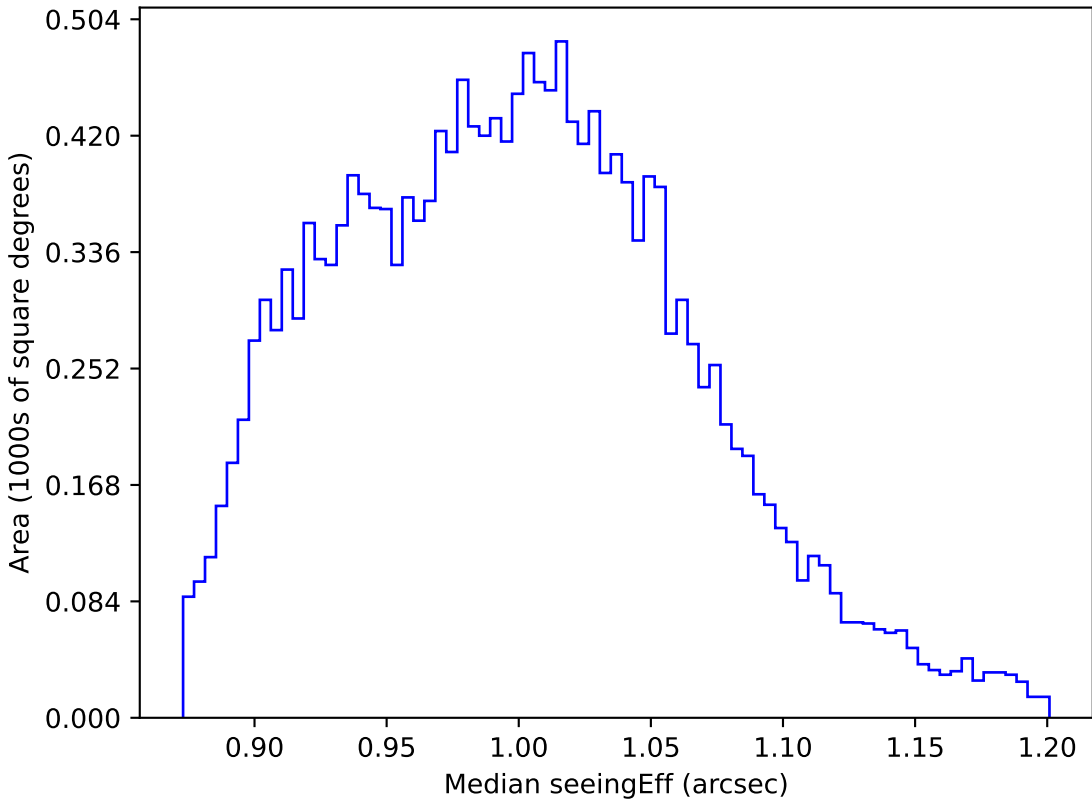
baseline_v3.5_10yrs WFD y band: Median seeingEff
