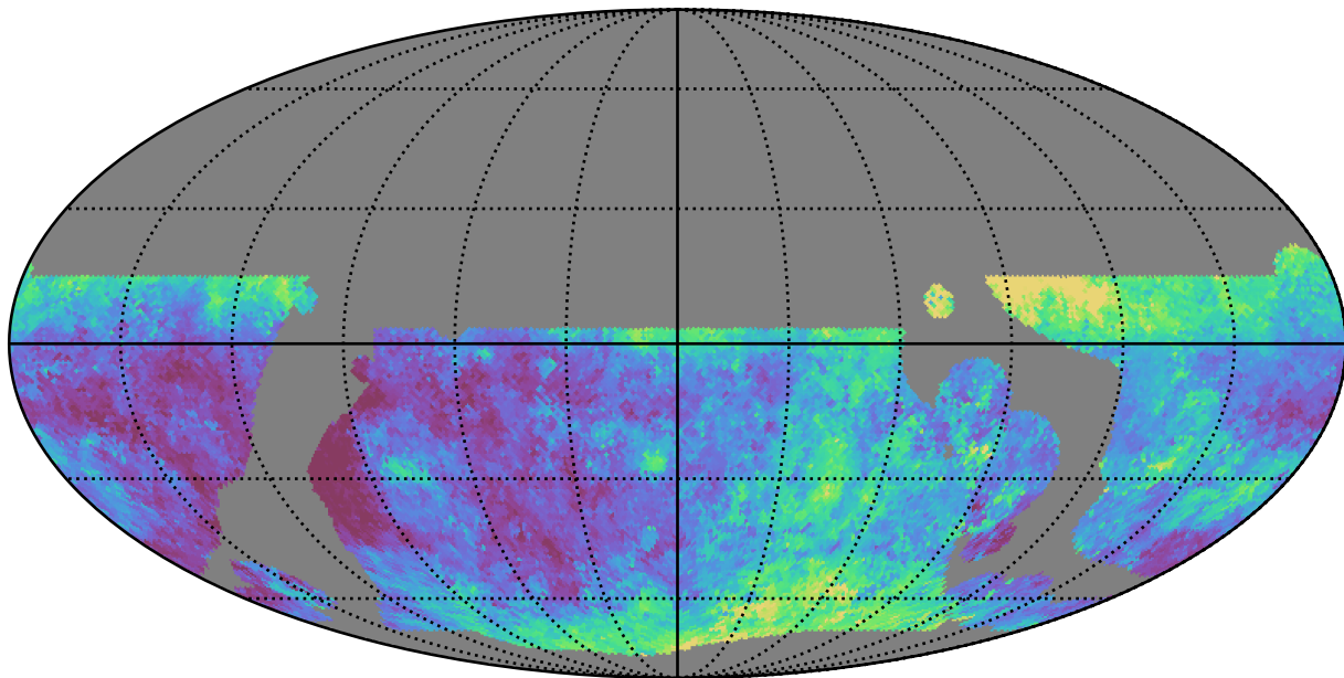
baseline_v3.5_10yrs WFD u band: Median seeingEff
