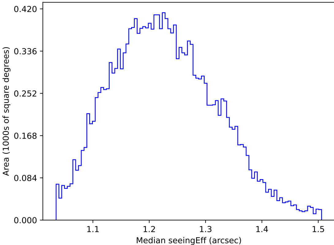
baseline_v3.5_10yrs WFD u band: Median seeingEff
