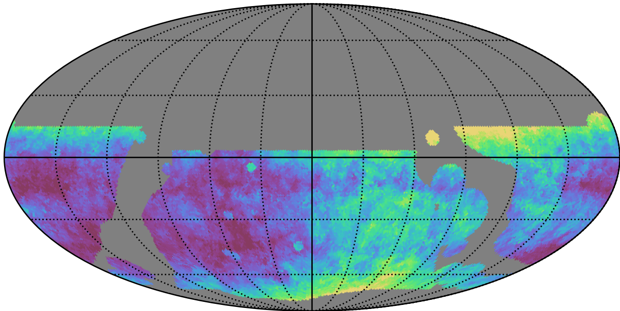
baseline_v3.5_10yrs WFD r band: Median seeingEff
