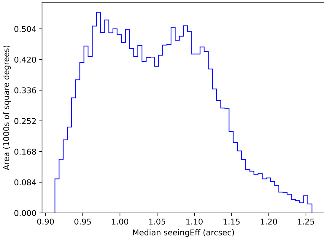
baseline_v3.5_10yrs WFD r band: Median seeingEff
