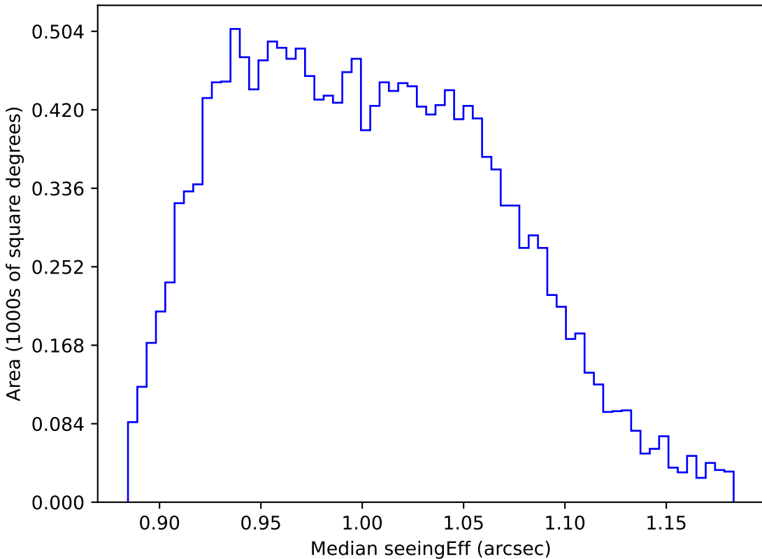
baseline_v3.5_10yrs WFD i band: Median seeingEff
