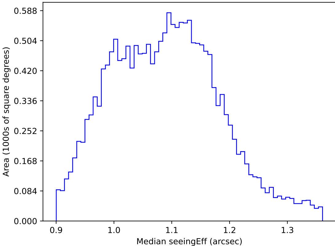
baseline_v3.5_10yrs WFD g band: Median seeingEff
