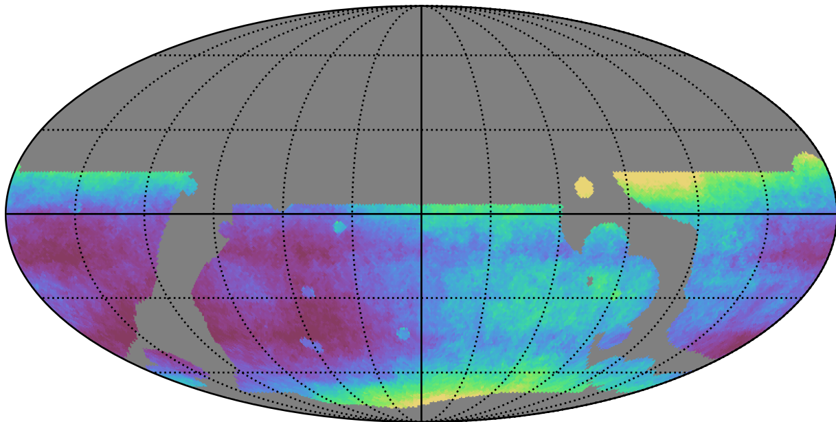
baseline_v3.5_10yrs WFD all bands: Median seeingEff
