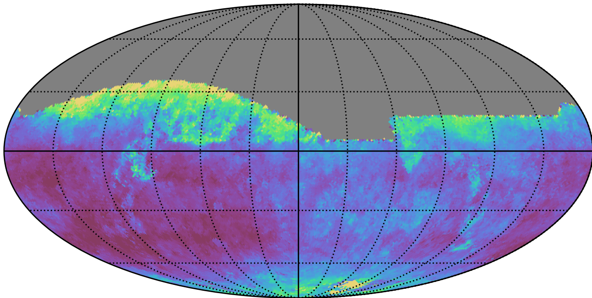
baseline_v3.5_10yrs All sky z band: Median seeingEff
