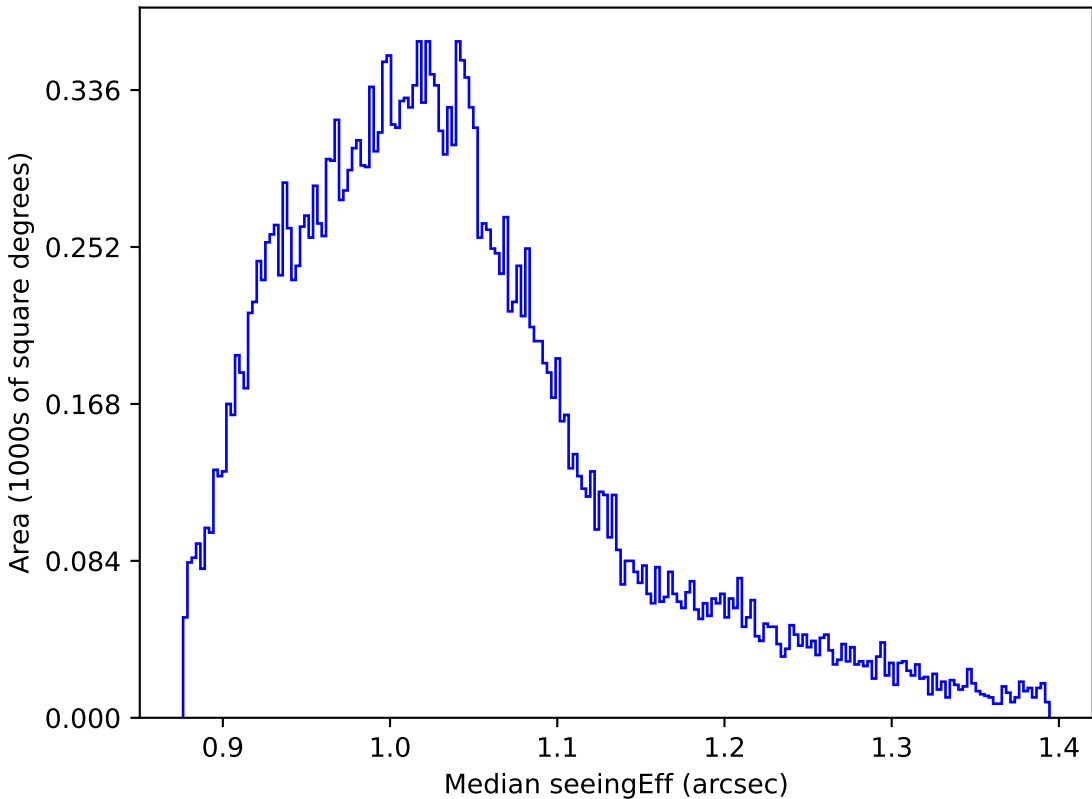
baseline_v3.5_10yrs All sky z band: Median seeingEff
