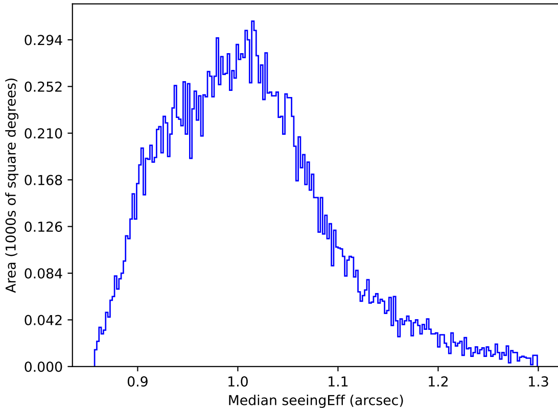
baseline_v3.5_10yrs All sky y band: Median seeingEff
