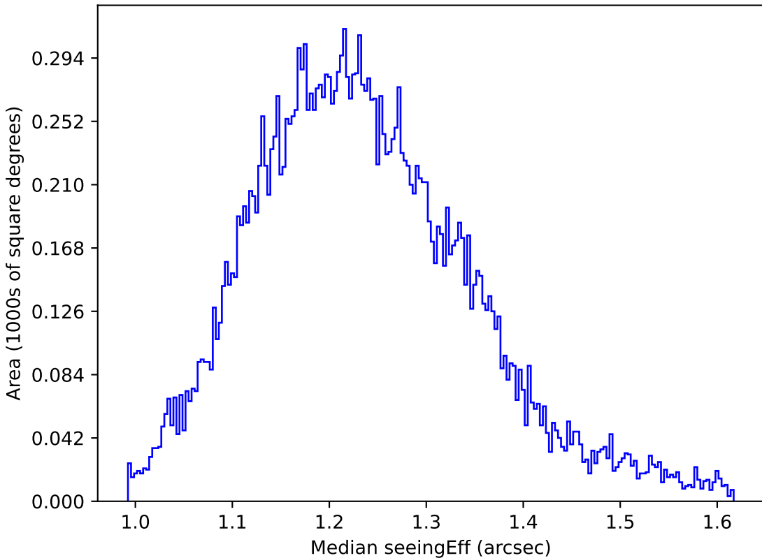
baseline_v3.5_10yrs All sky u band: Median seeingEff
