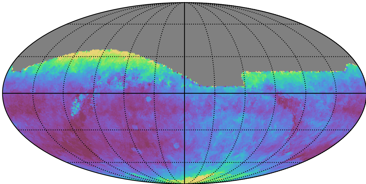
baseline_v3.5_10yrs All sky r band: Median seeingEff
