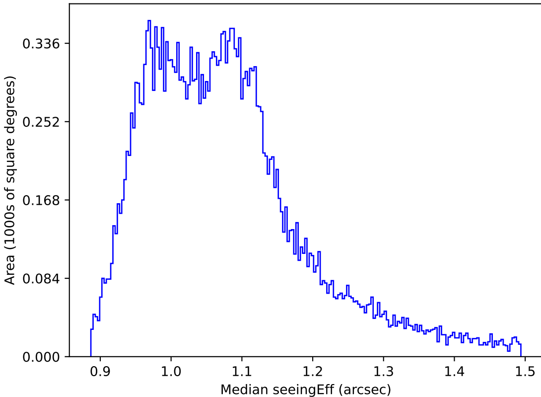
baseline_v3.5_10yrs All sky r band: Median seeingEff
