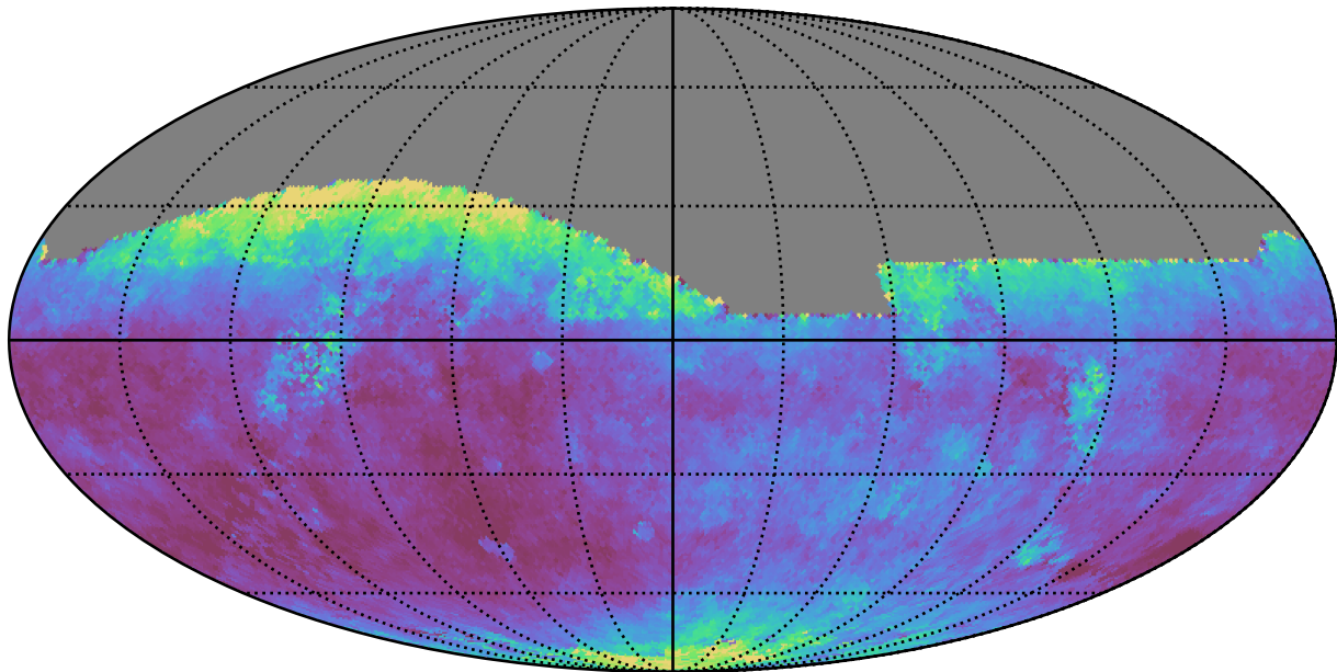
baseline_v3.5_10yrs All sky i band: Median seeingEff
