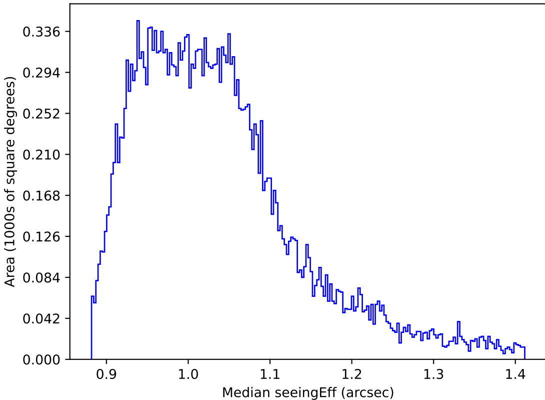
baseline_v3.5_10yrs All sky i band: Median seeingEff
