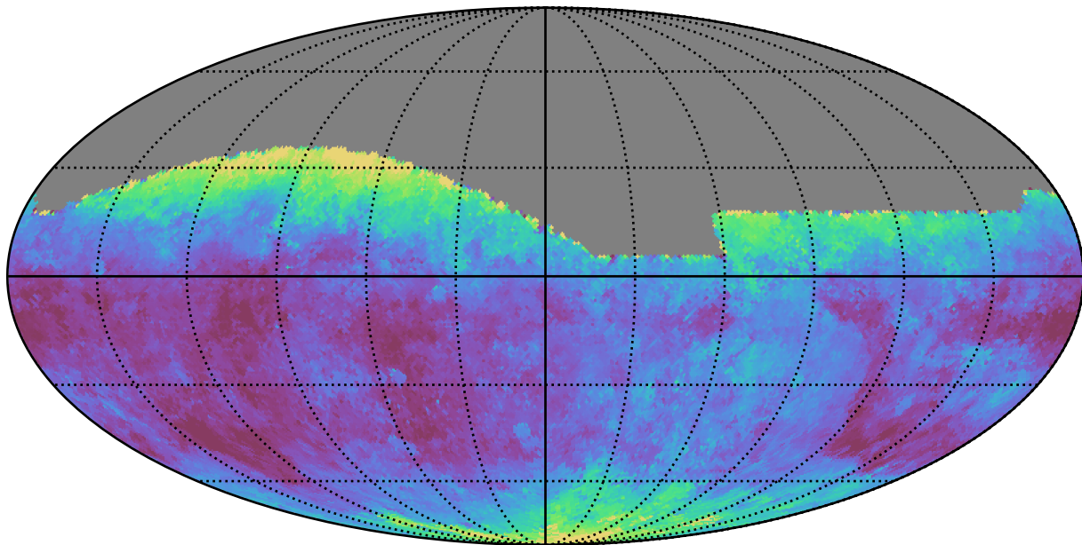
baseline_v3.5_10yrs All sky g band: Median seeingEff
