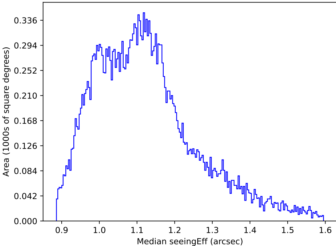
baseline_v3.5_10yrs All sky g band: Median seeingEff
