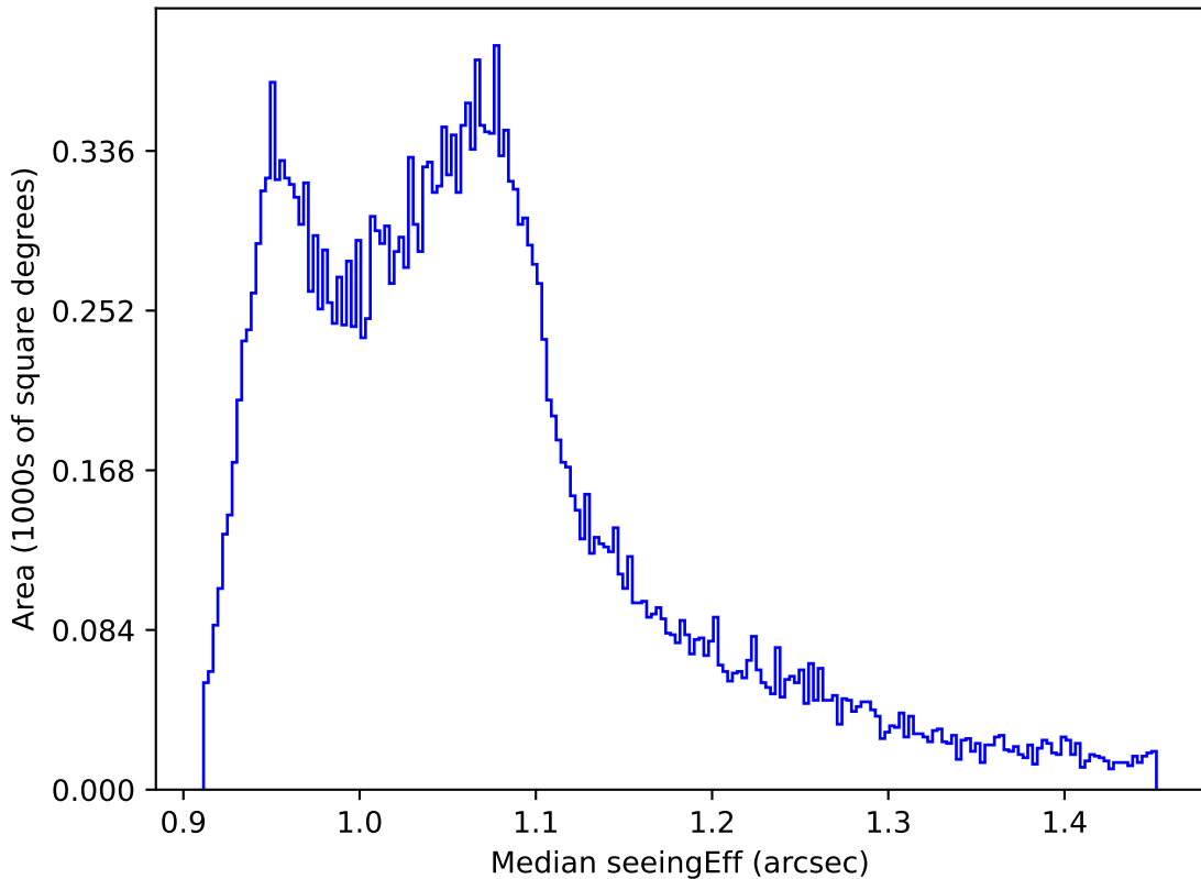
baseline_v3.5_10yrs All sky all bands: Median seeingEff
