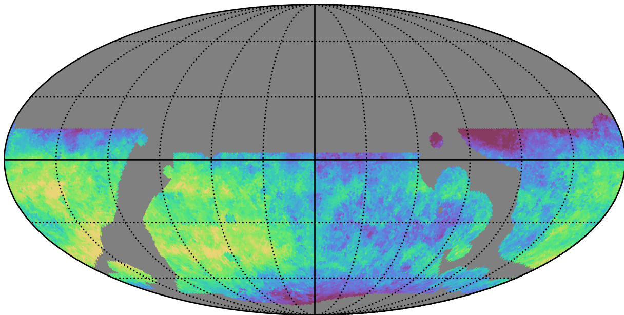
baseline_v3.5_10yrs WFD z band: Median saturation_mag
