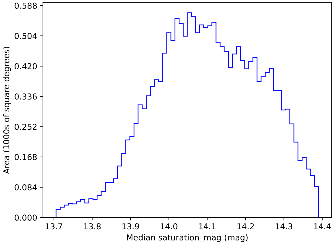
baseline_v3.5_10yrs WFD z band: Median saturation_mag
