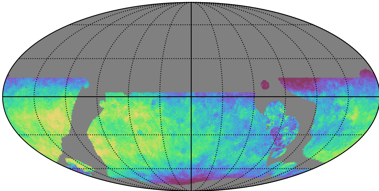
baseline_v3.5_10yrs WFD y band: Median saturation_mag
