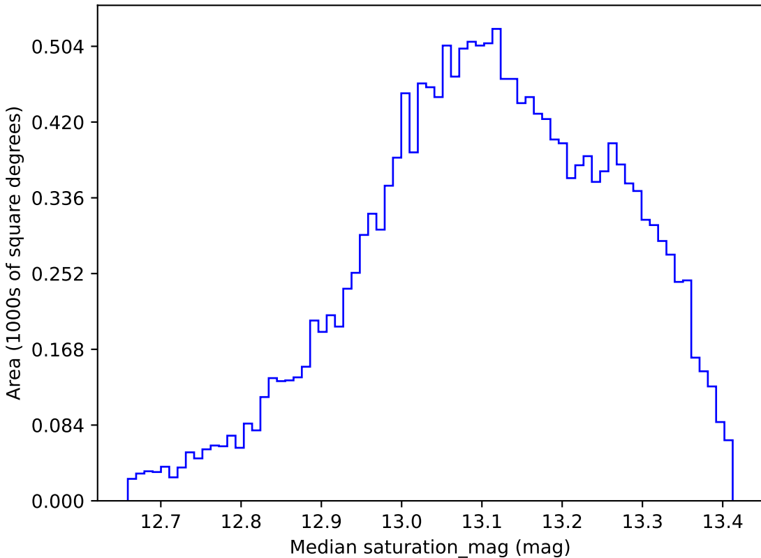
baseline_v3.5_10yrs WFD y band: Median saturation_mag
