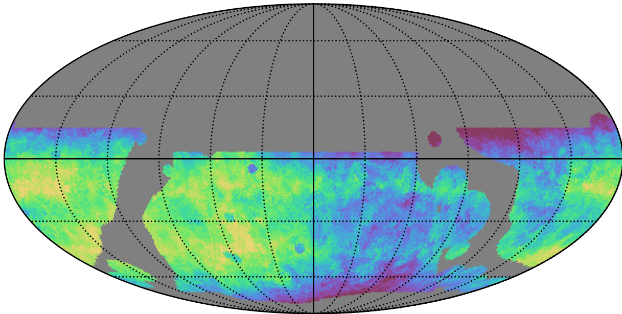
baseline_v3.5_10yrs WFD r band: Median saturation_mag
