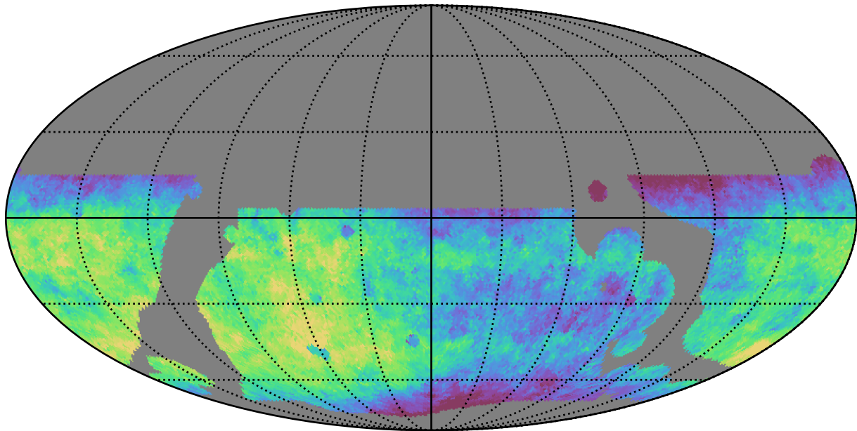
baseline_v3.5_10yrs WFD i band: Median saturation_mag
