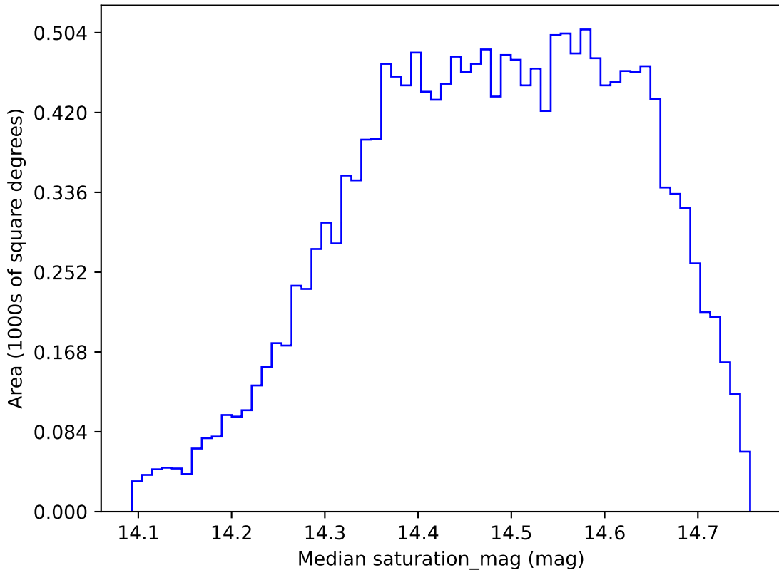
baseline_v3.5_10yrs WFD i band: Median saturation_mag
