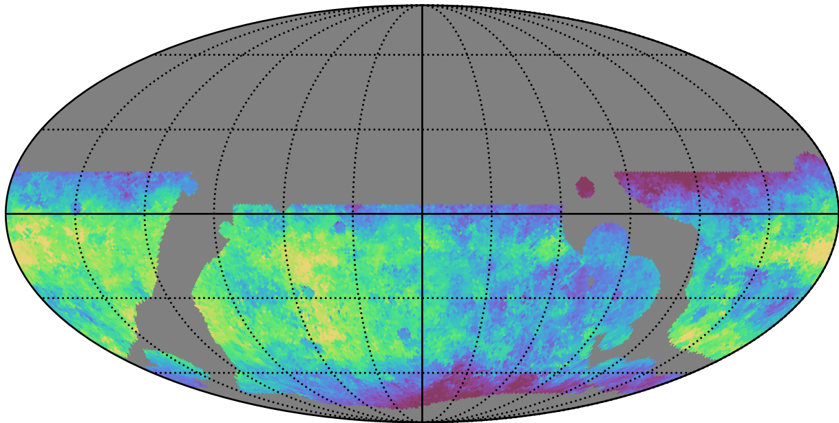
baseline_v3.5_10yrs WFD g band: Median saturation_mag
