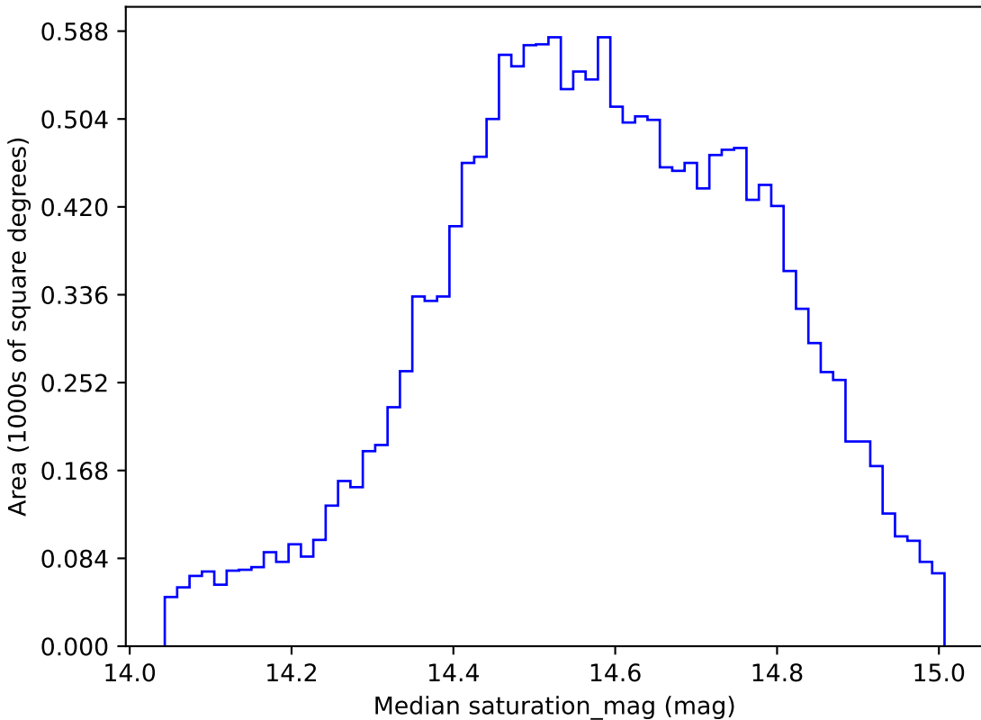
baseline_v3.5_10yrs WFD g band: Median saturation_mag
