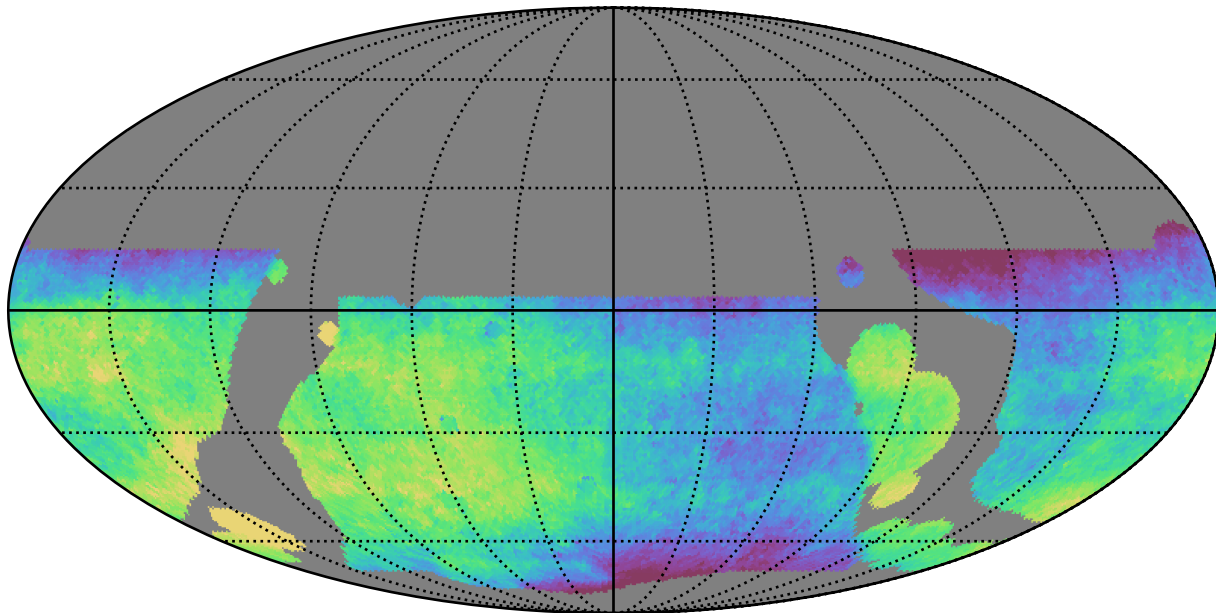
baseline_v3.5_10yrs WFD all bands: Median saturation_mag
