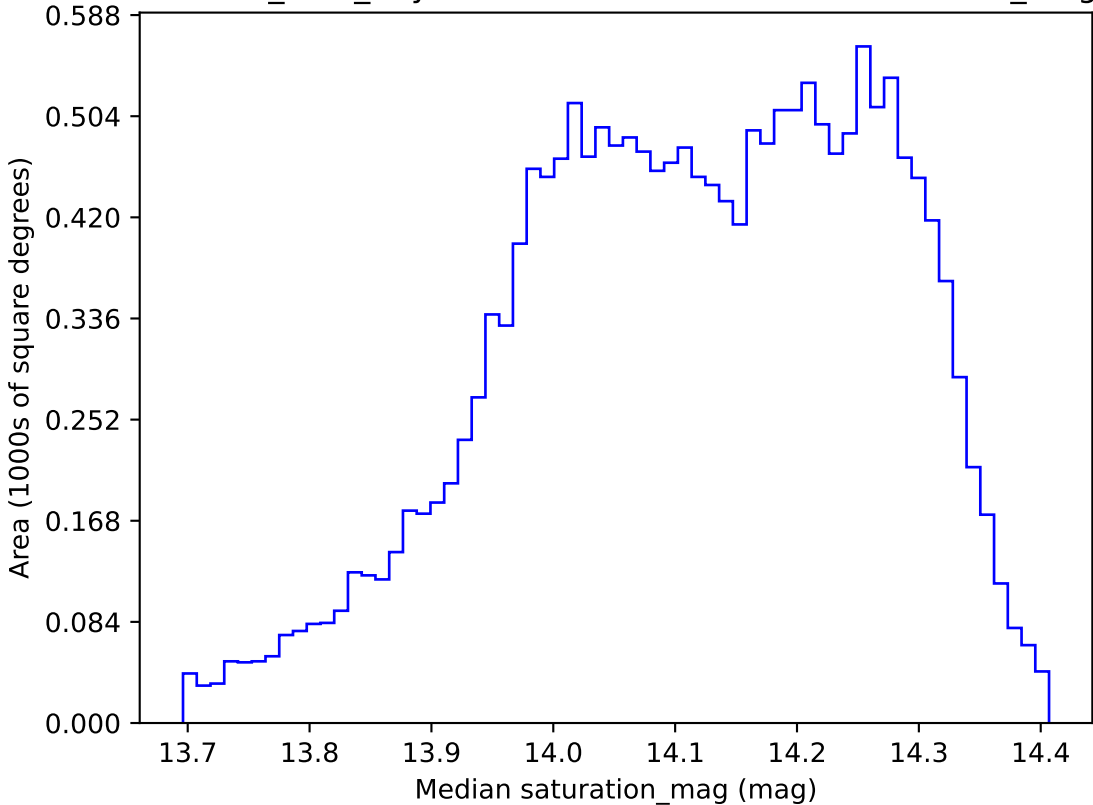
baseline_v3.5_10yrs WFD all bands: Median saturation_mag
