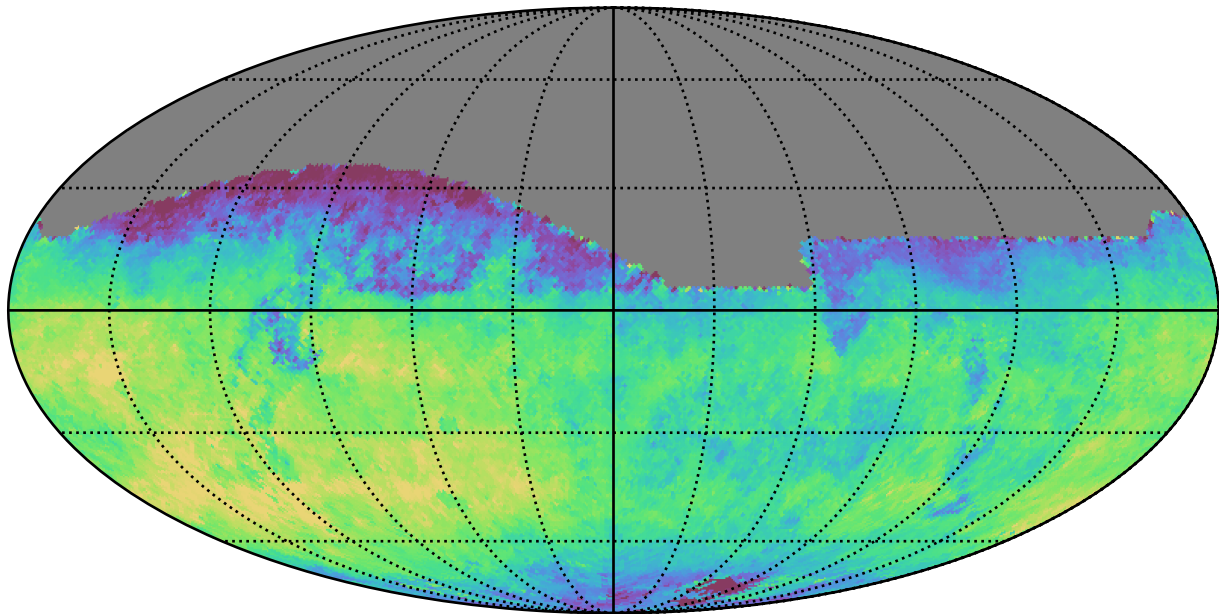
baseline_v3.5_10yrs All sky z band: Median saturation_mag
