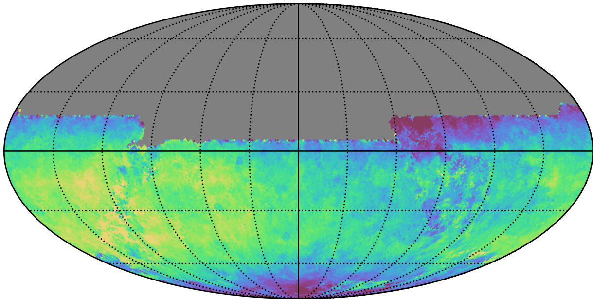
baseline_v3.5_10yrs All sky y band: Median saturation_mag
