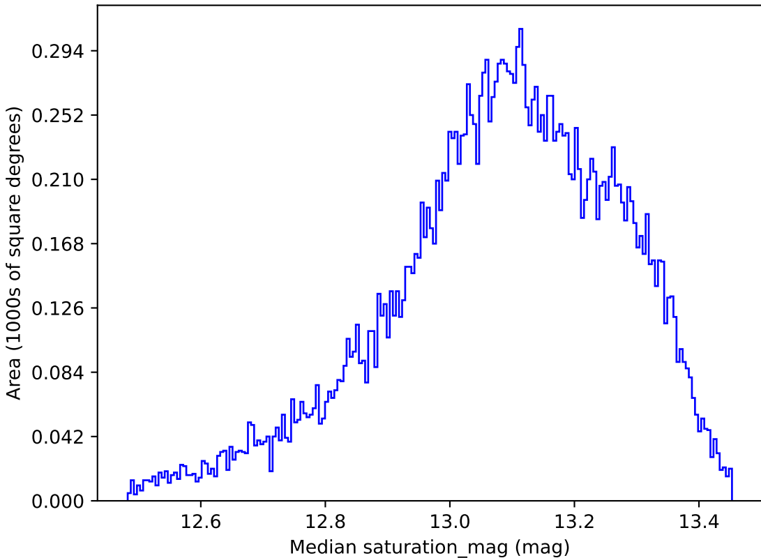
baseline_v3.5_10yrs All sky y band: Median saturation_mag
