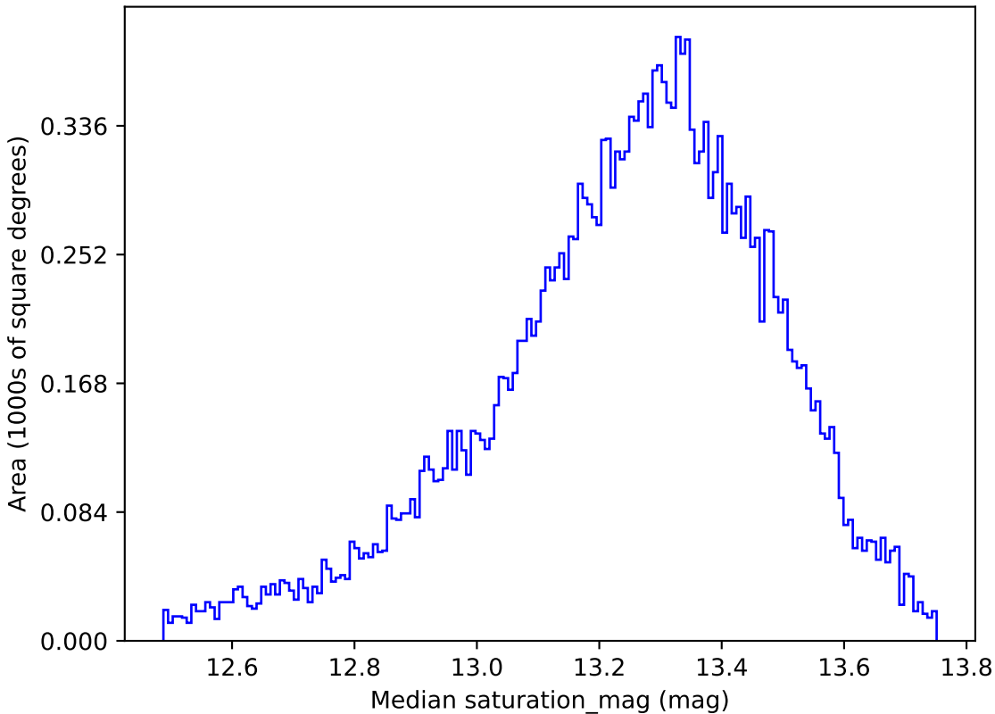
baseline_v3.5_10yrs All sky u band: Median saturation_mag
