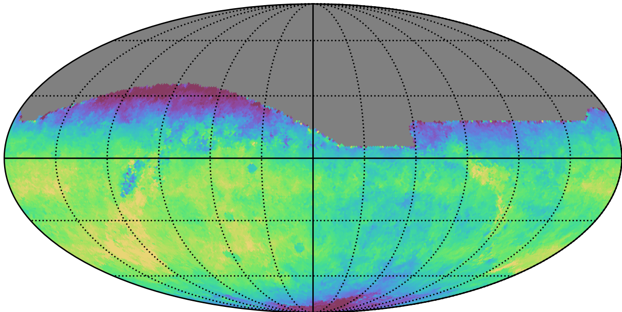
baseline_v3.5_10yrs All sky r band: Median saturation_mag
