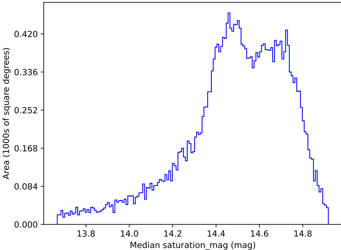
baseline_v3.5_10yrs All sky r band: Median saturation_mag
