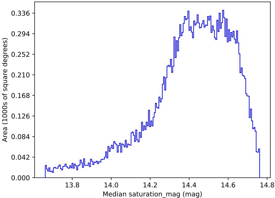
baseline_v3.5_10yrs All sky i band: Median saturation_mag
