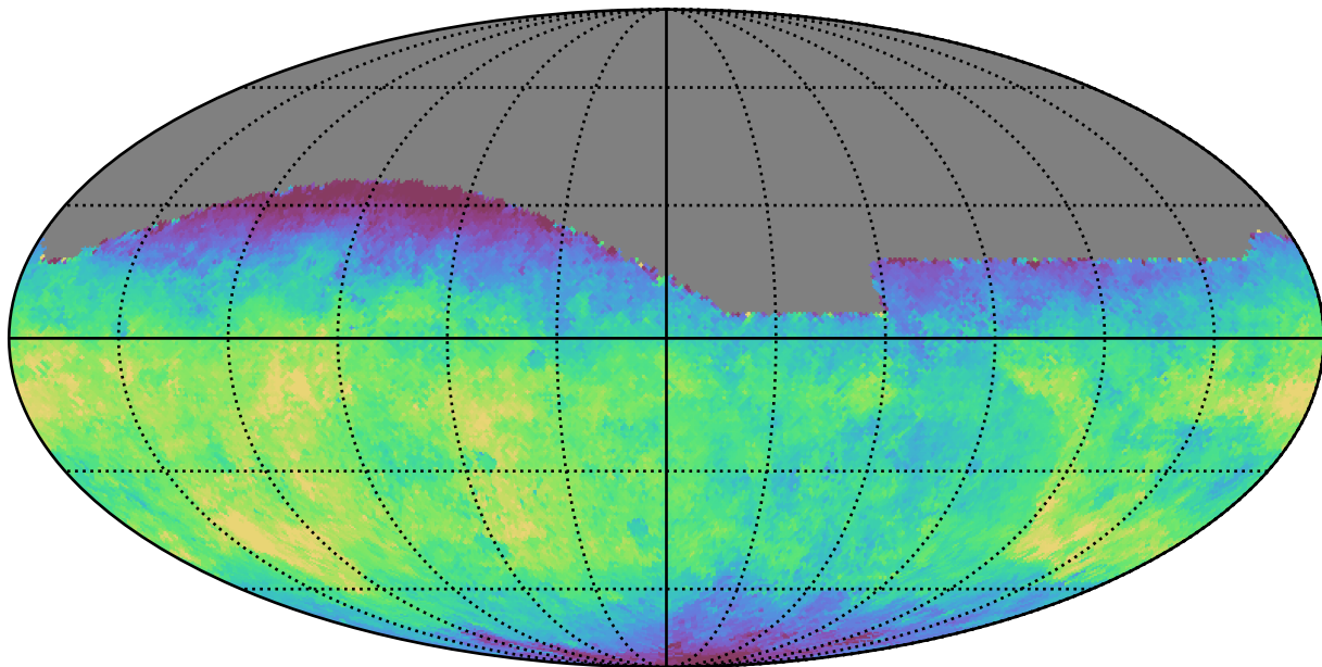
baseline_v3.5_10yrs All sky g band: Median saturation_mag
